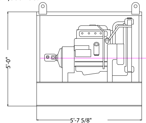
REMOTE HYDRAULIC POWER PACK 40 HP DIESEL ENGINE-TO- 25 GPM PUMP W/ ELECTRIC STARTER.
